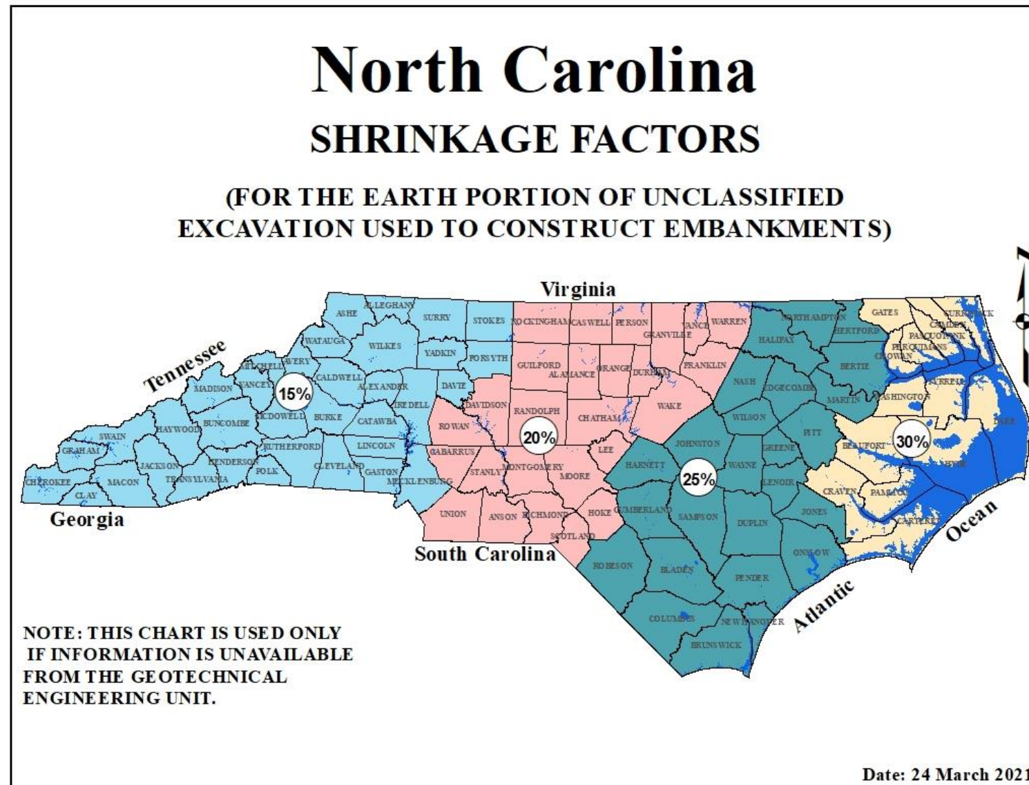
Figure 15-1 Shrinkage Factors
