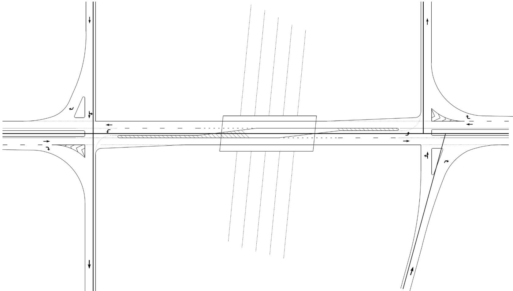
Figure 9-8b Ramp Terminal Design (Alternate)
