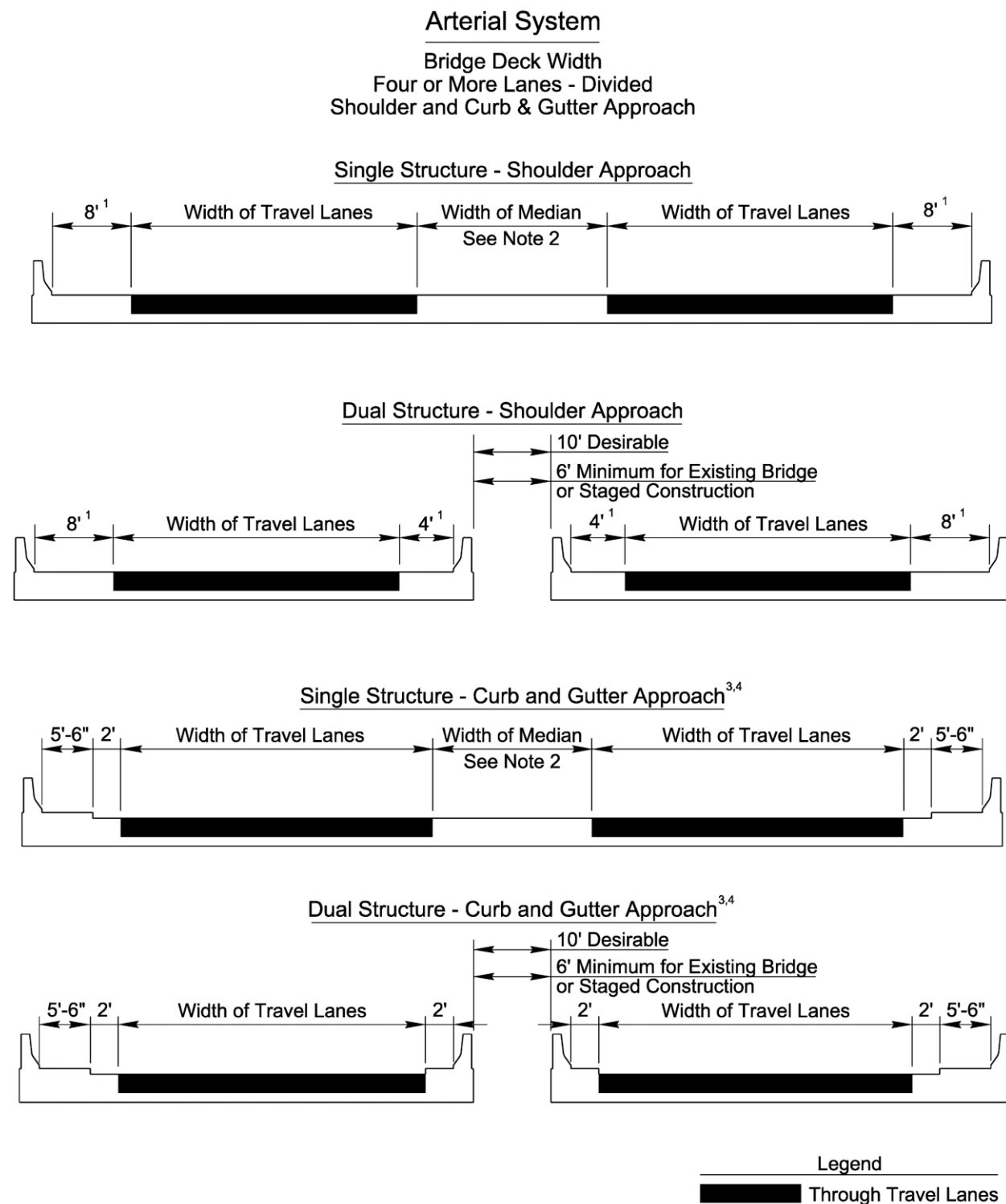
Figure 5-4 Arterial System Bridge Deck Widths for Four or More Lanes Divided Shoulder Approach and Curb and Gutter Approach
