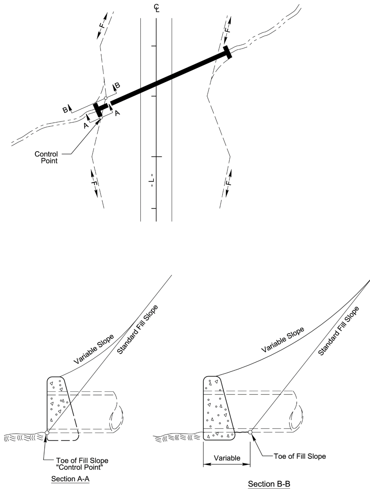
Figure 7-5 Example of Endwall Treatment
