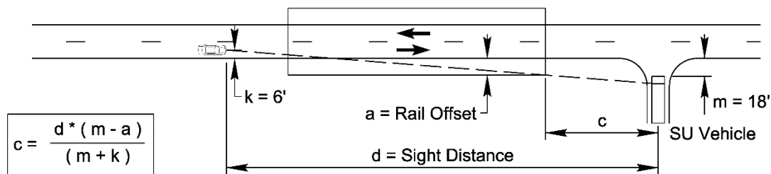
Figure 9-6 Design Requirements for Crossroad Sight Distance at Interchanges, Single Unit Vehicle Criteria
