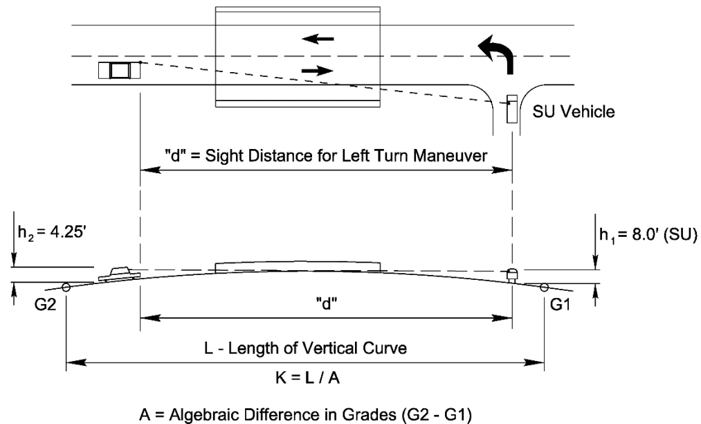
Figure 9-5 Vertical Sight Distance Control for Crest Curves at Interchanges, Single Unit Vehicle Criteria
