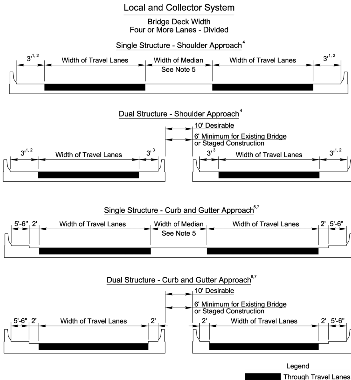
Figure 5-9 Local and Collector System Bridge Deck Widths for Four or More Lanes Divided
