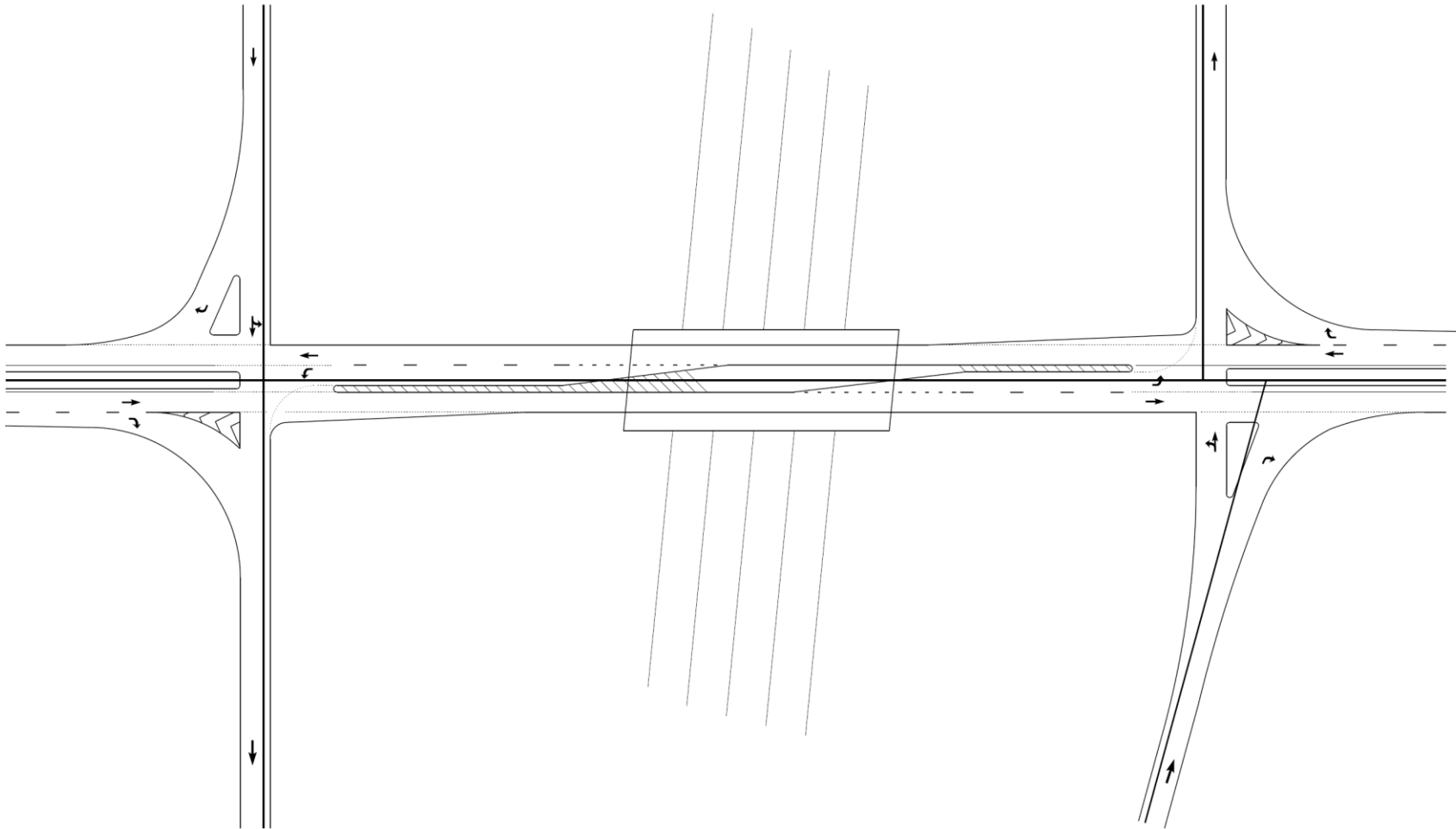
Figure 9-8a Ramp Terminal Design (Recommended)
