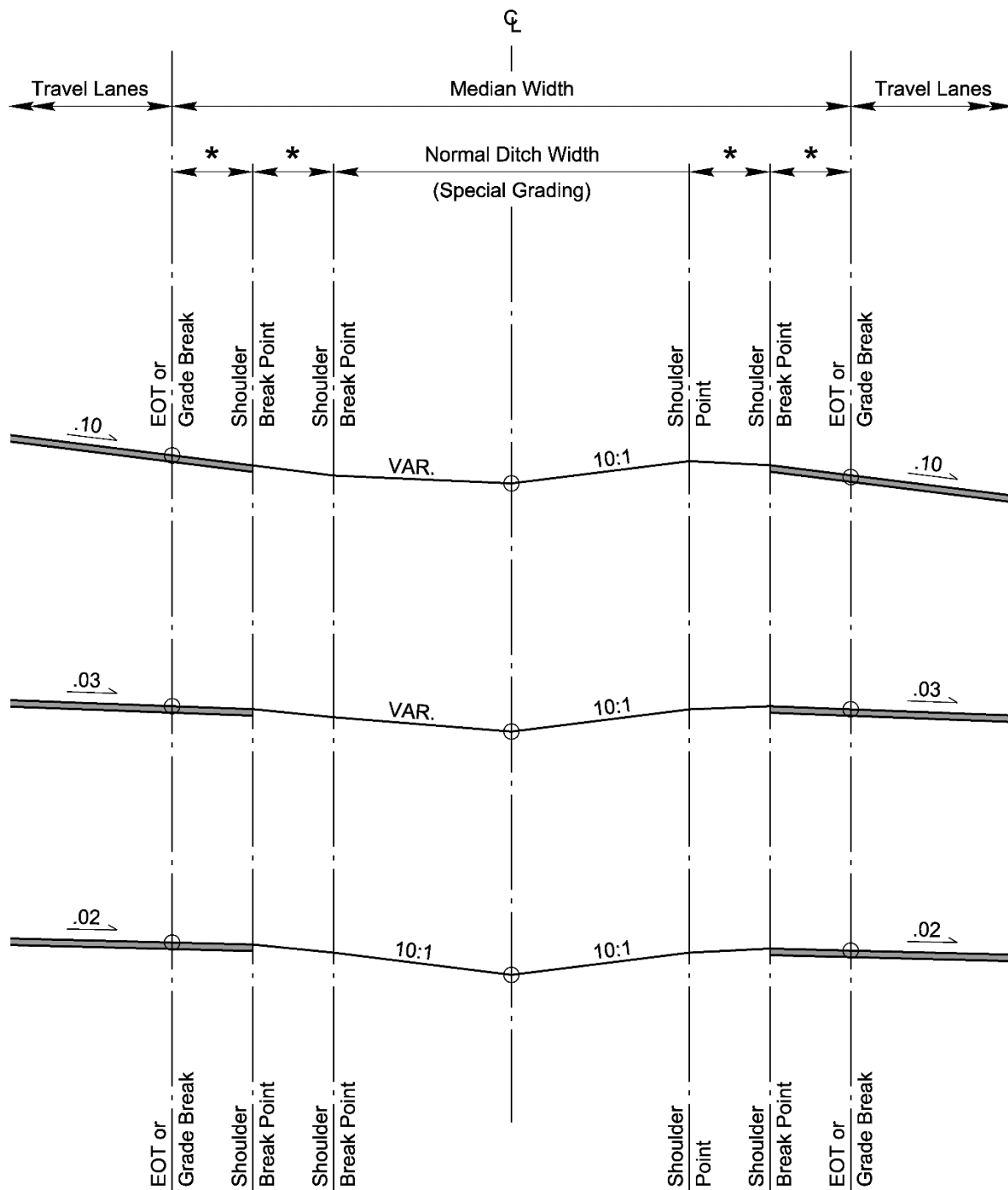
Figure 6-6 Special Grading in Superelevated Location
