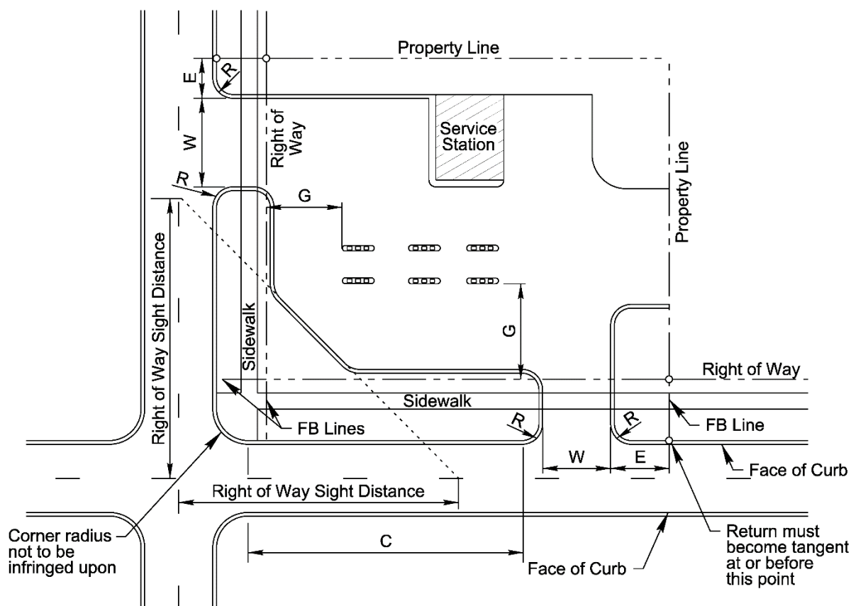
Figure 10-4 Example Driveway Scenario for Corner Business
