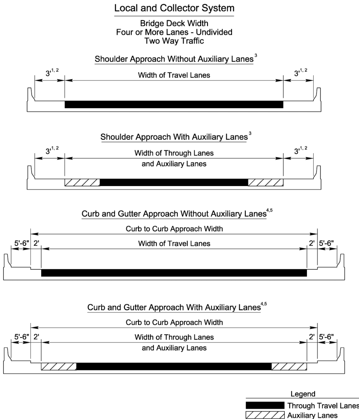
Figure 5-11 Local and Collector System Bridge Deck Widths for Four or More Lanes Undivided Two-Way Traffic
