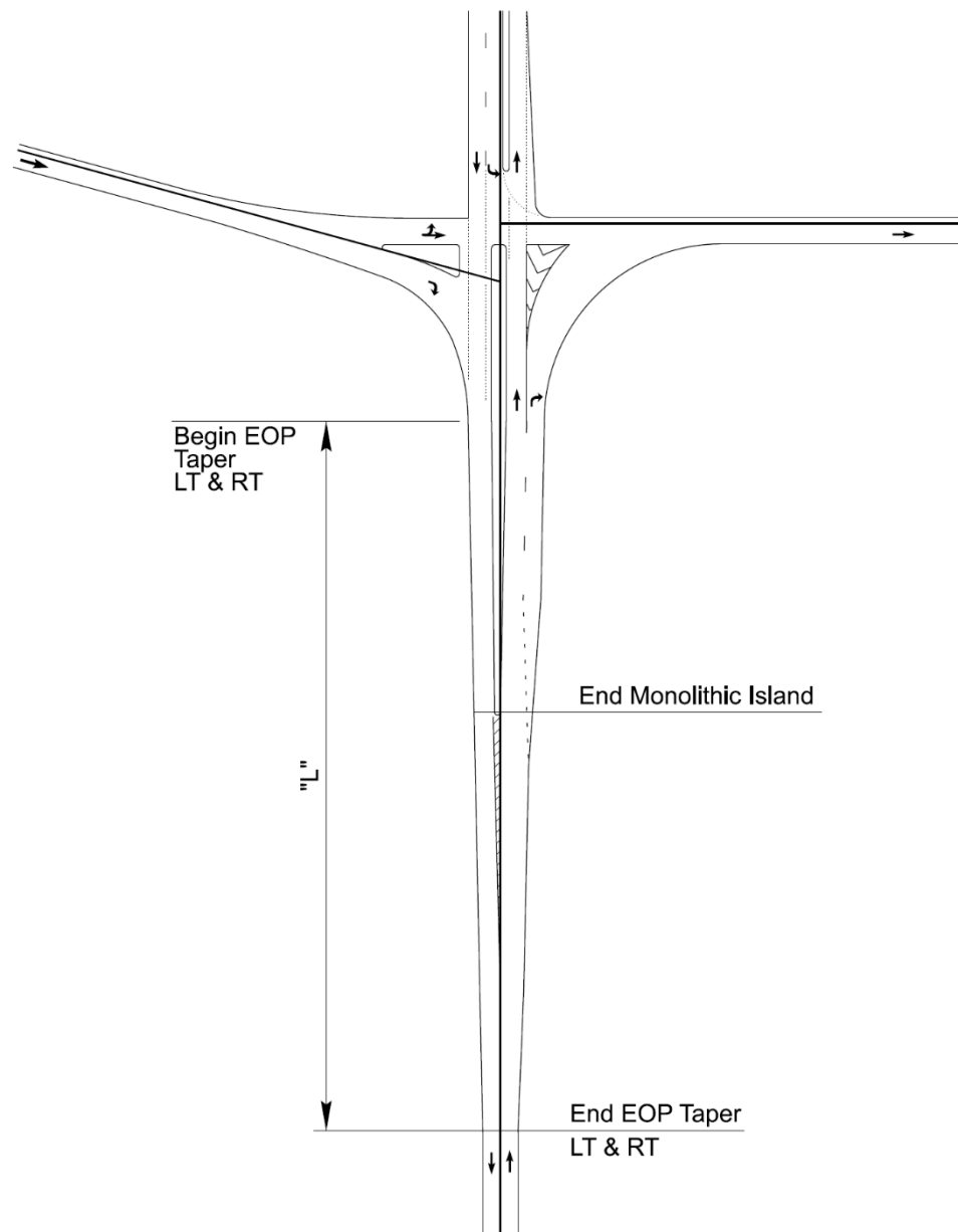
Figure 9-7b Y- Line Transition at Ramp Terminal for Three-Lane -Y- Line Section (Alternate)
