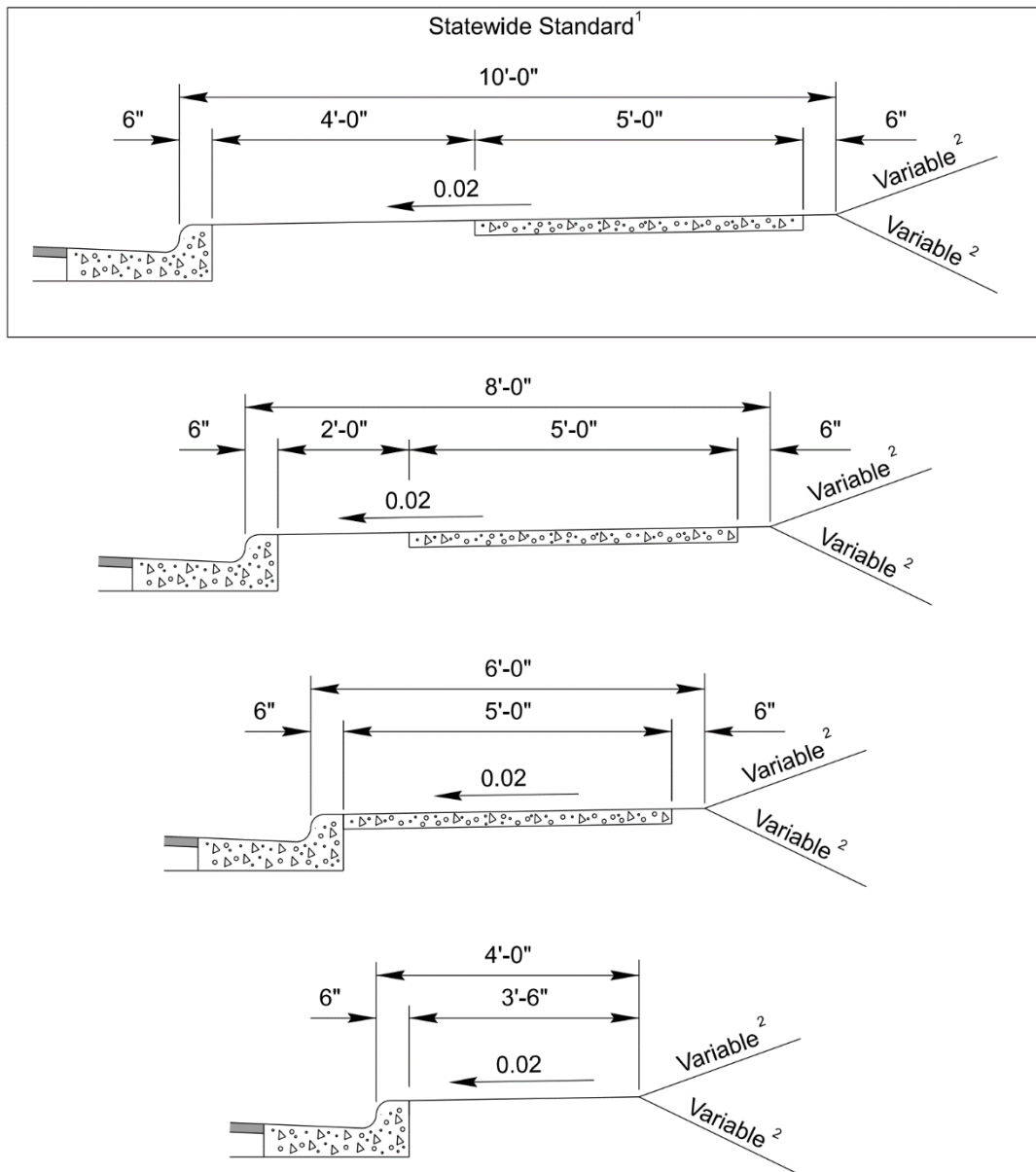
Figure 4-6 Berm Width
