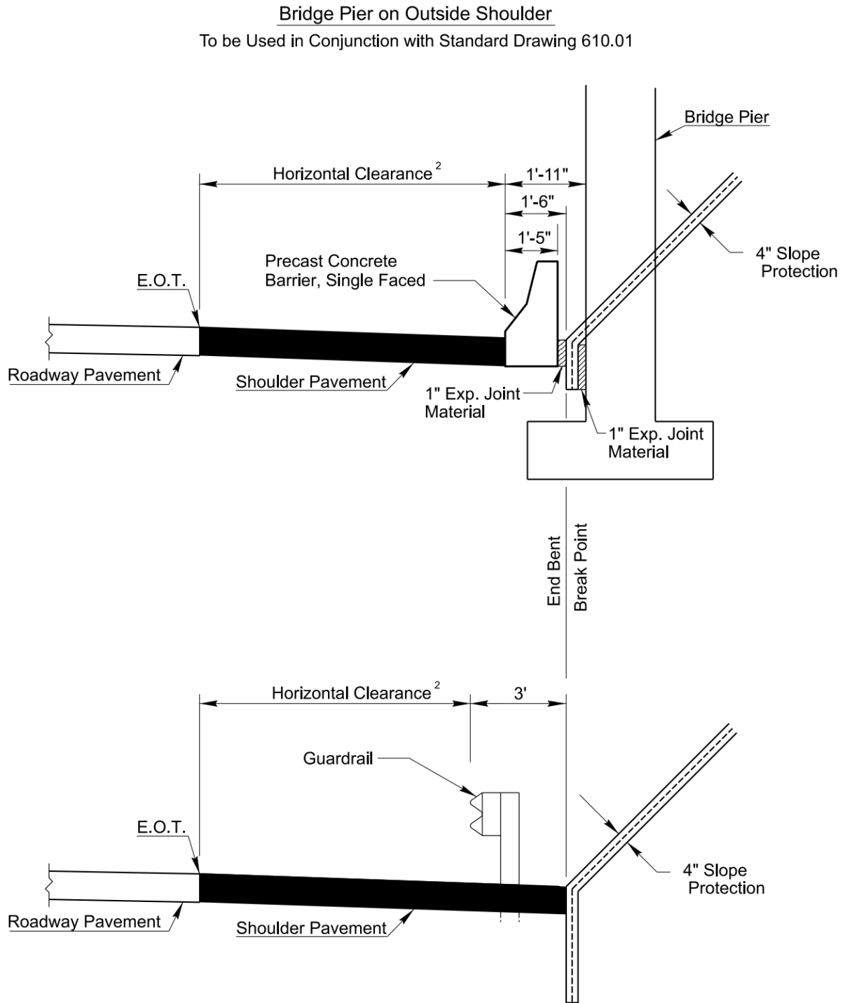
Guardrail on Outside Shoulder To be Used in Conjunction with Standard Drawing 610.02
