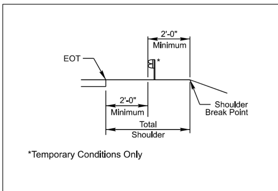
Figure 6-5 Minimum Offsets for Temporary Guardrail Placement
