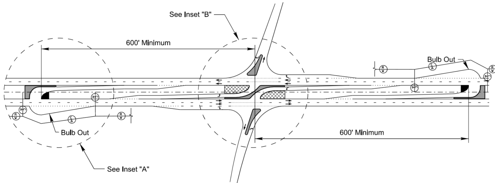
Figure 8-2 Reduced Conflict Intersection
