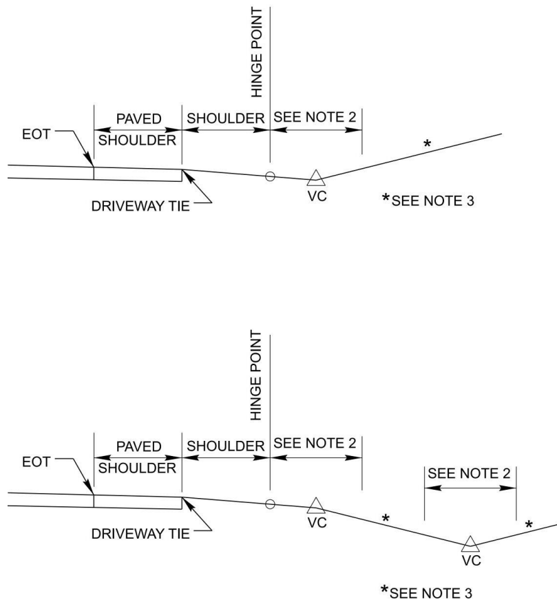
Figure 4-8 Commercial and Residential Driveway Profile
