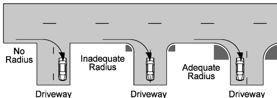
Figure 10-2 Intersection Turn Radii
