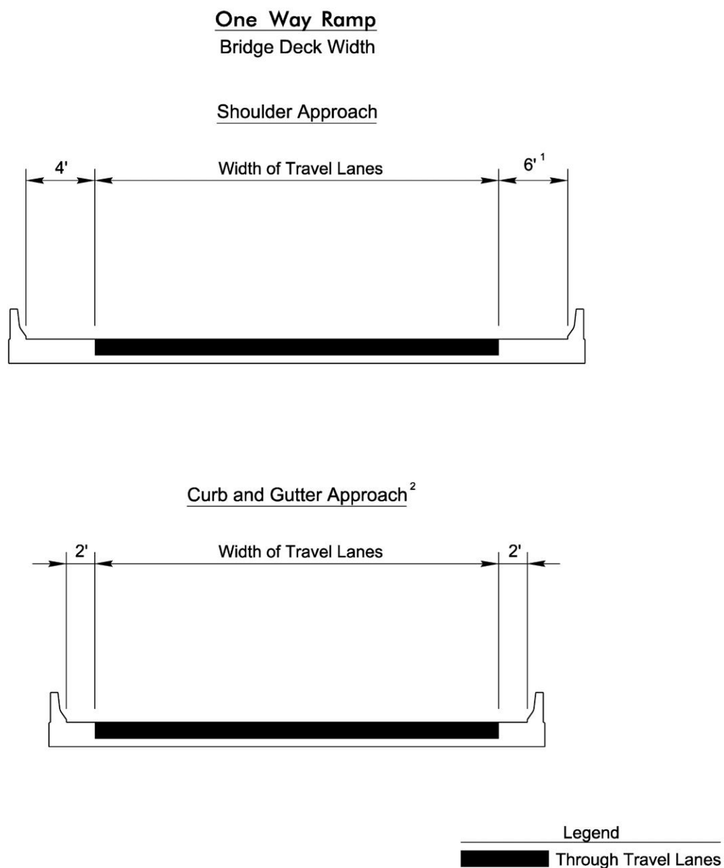
Figure 5-12 One Way Ramp Bridge Deck Widths
