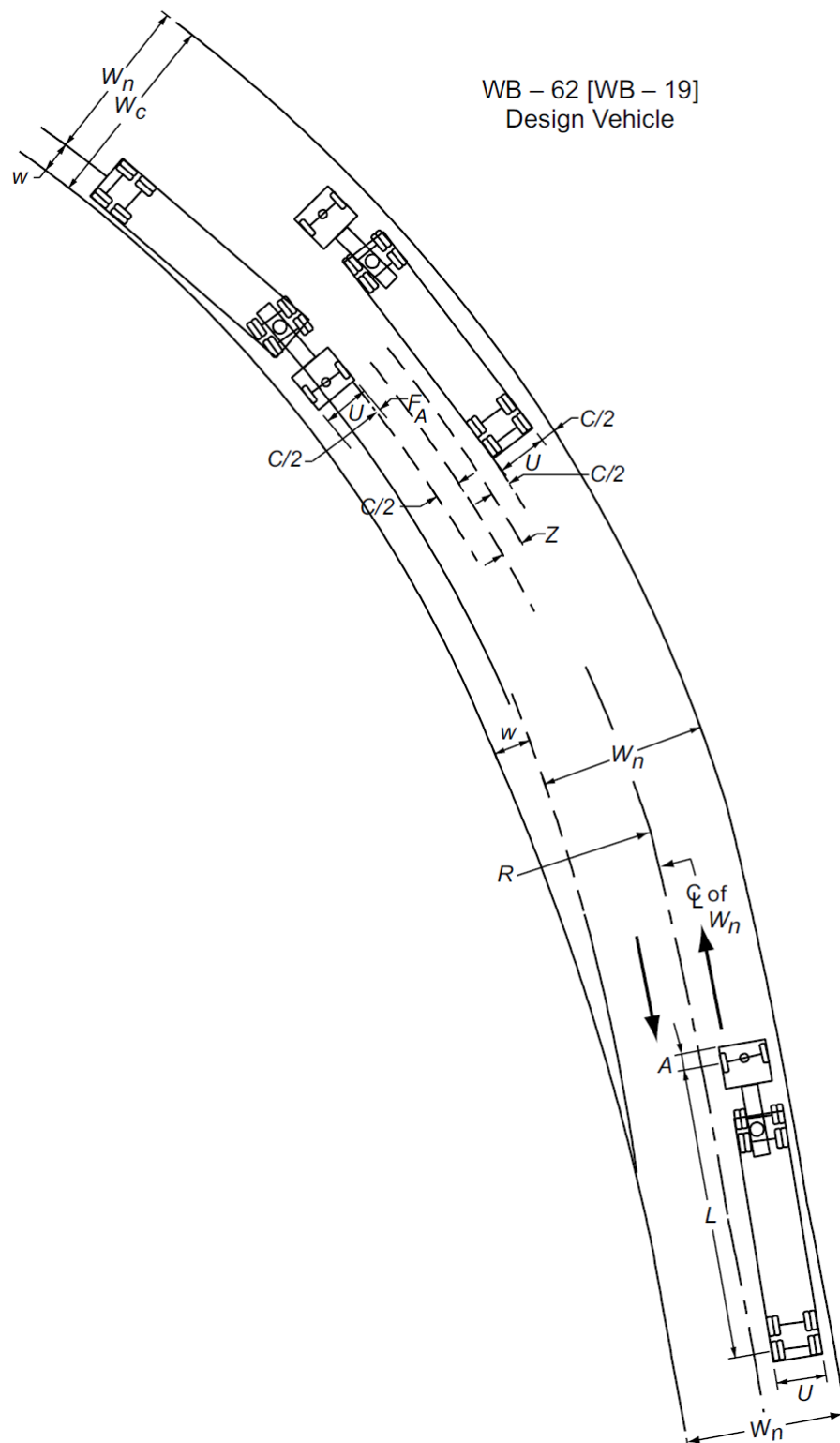
Figure 3-1 Widening Components on Open Highway Curves (Two-Lane Highways, One-Way or Two-Way)
