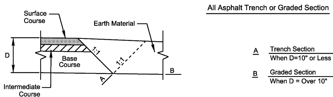
Figure 2-3 Pavement Edge Construction with Flexible Pavement
