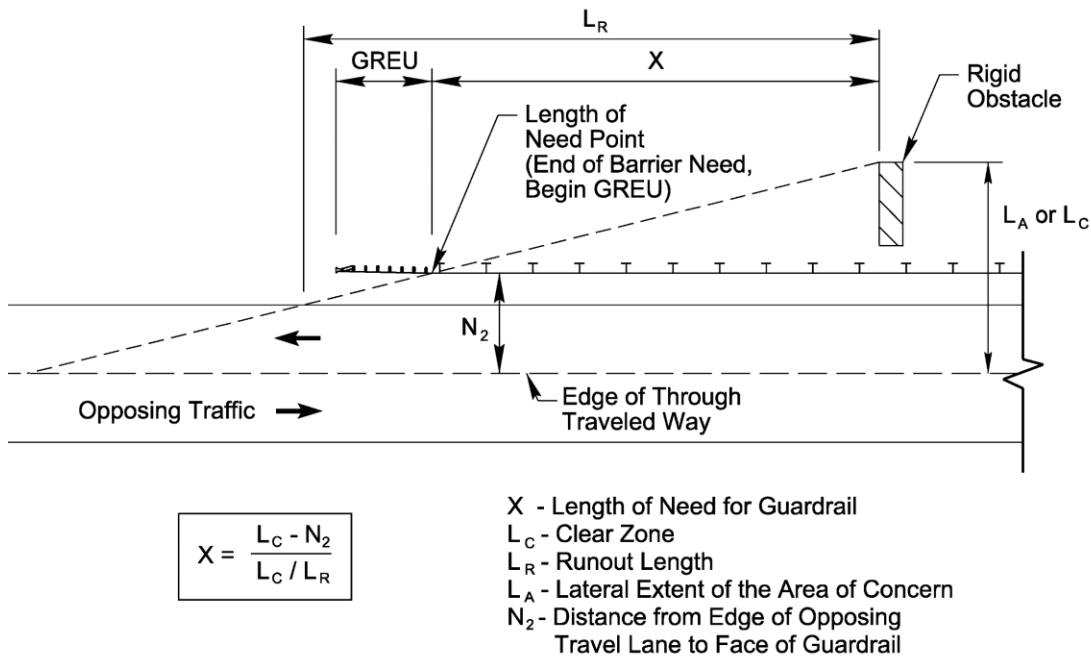
Figure 6-2 Detail of Guardrail Placement on Trailing End of Rigid Obstacle Warrant
