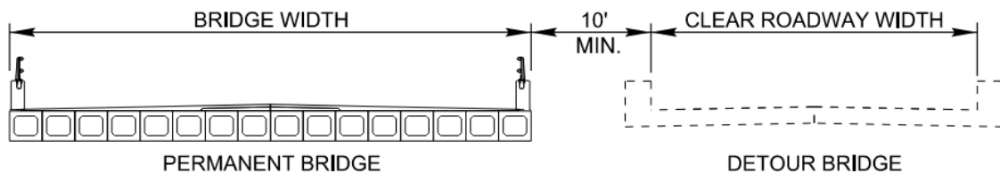
Figure 5-19 Minimum offset between Permanent and Detour Bridges
