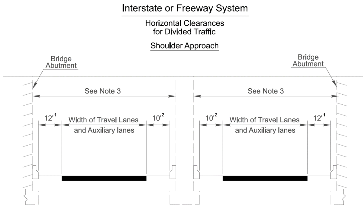
Figure 5-13 Interstate or Freeway System Horizontal Clearances for Divided Traffic
