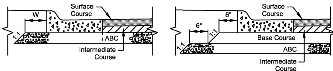
Figure 2-4 Pavement Edge Construction with Shoulder Drains
