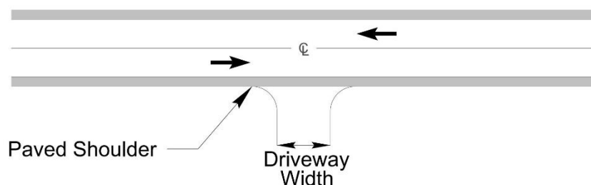
Figure 4-9 Driveways Tying to Paved Shoulders
