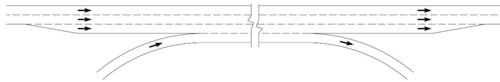
Figure 9-2 Adding Auxiliary Lanes for Improved Weaving Operations
