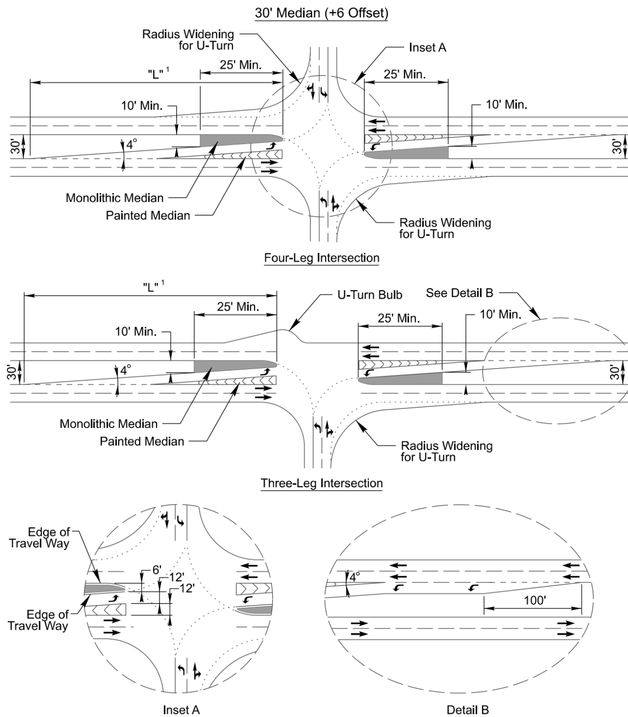
Figure 8-13 Guidelines for Offsetting Opposing Left Turn Lanes on Divided Roadways with a 30' Median
