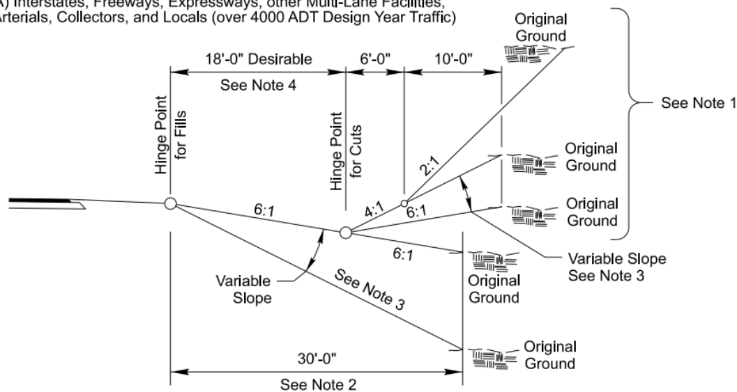
Figure 4-4 Criteria for Roadway Typical Section and Slopes
