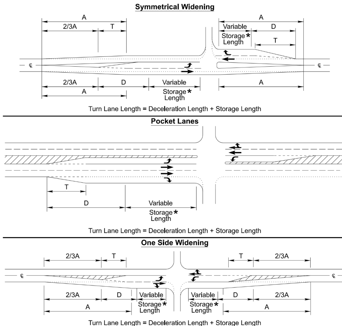
Figure 8-11 Recommended Treatment for Turn Lanes
