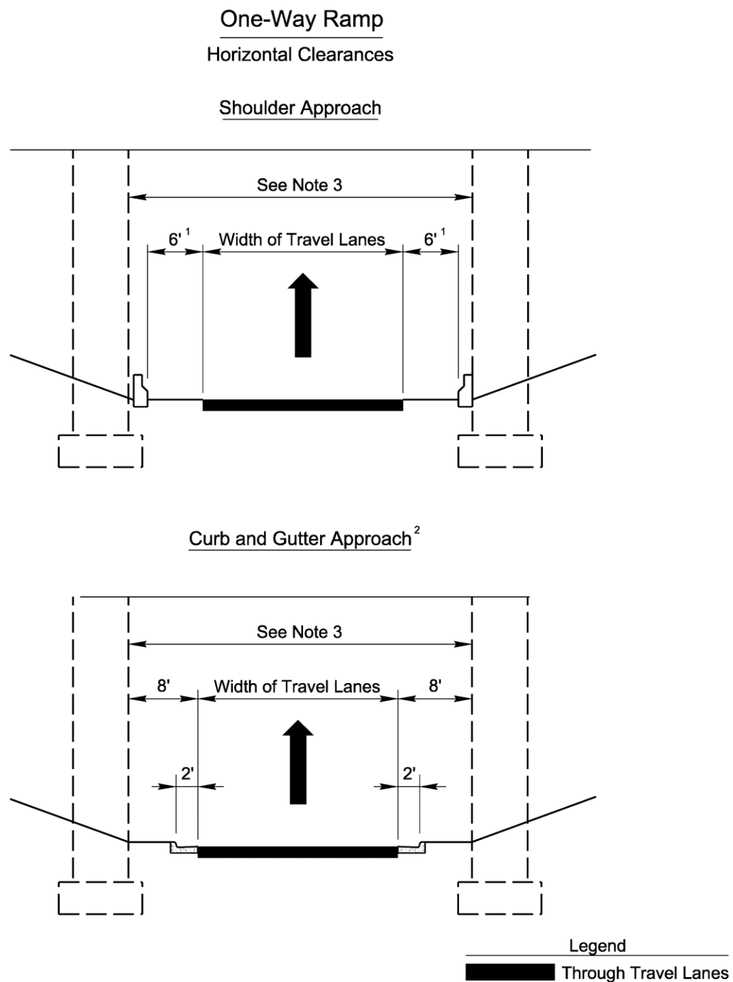
Figure 5-18 One Way Ramp Horizontal Clearances
